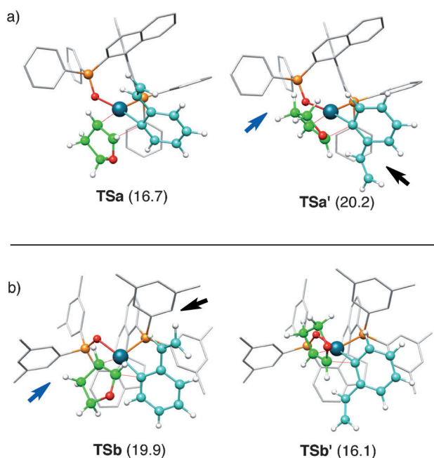
Figure 2. Transition states and energies (kcal mol -1 ) of 2,3-dihydrofuran insertion into cationic [L](alkene)(o-vinylphenyl)Pd II complexes. L is (R)-binap(O) in (a) and (R)-Xyl-SDP(O) in (b). Close contacts are indicated with arrows. To account for the dispersive effect in the cationic transition states, calculations were performed with a large basis set: M06-2X/[LANL2TZ(f)(Pd),6-31+G*(others)]//B3LYP/[LANL2DZ(Pd),6-31G*(O,P),6-31G(H,C)]. The solvent effect of 1,4-dioxane was taken into account by the polarizable continuum model (PCM) method.
